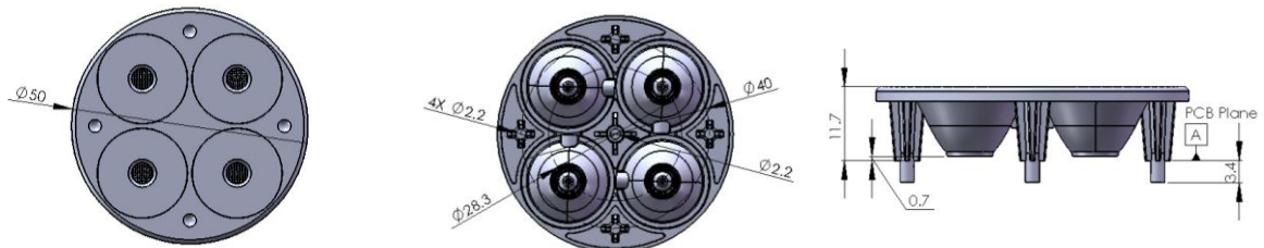
Figure 2: FLP4 layout and dimensions (Mechanical CAD files available)
