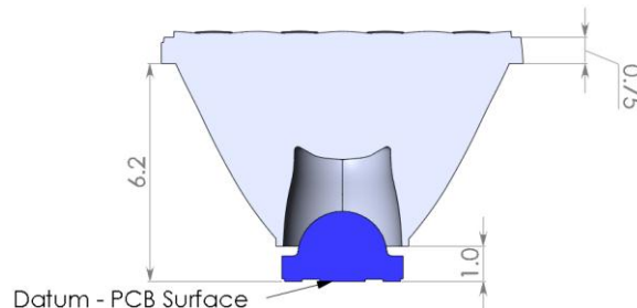
Figure 2. Lens cross section showing the correct vertical mounting position
